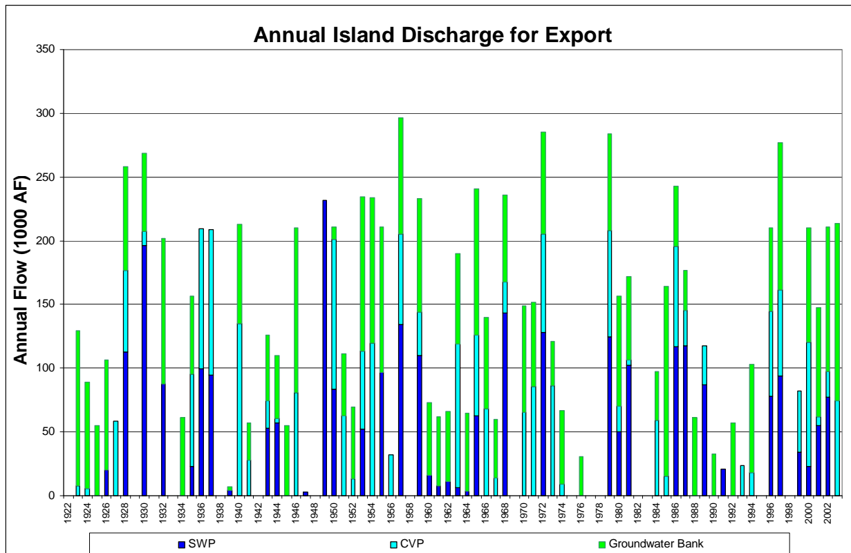
Figure A-16. Example Annual Plot of Island Discharge for Export from the Ann_plot Worksheet
