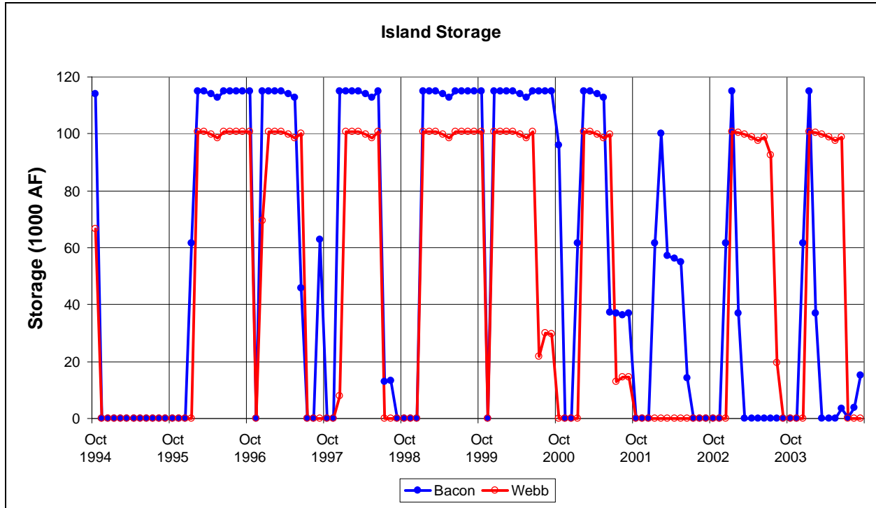
Figure A-15. Example Plot of Monthly Island Storage from the TS_plot Worksheet
